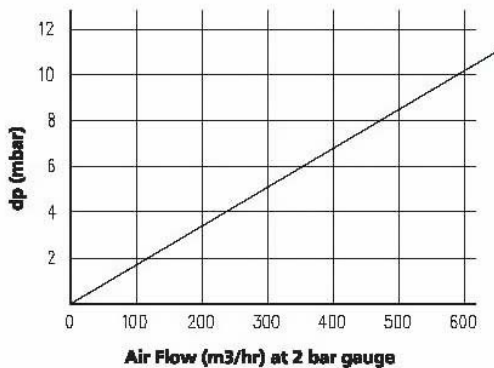
Pressure Drop Graph for Transflow Filter/Size 3
